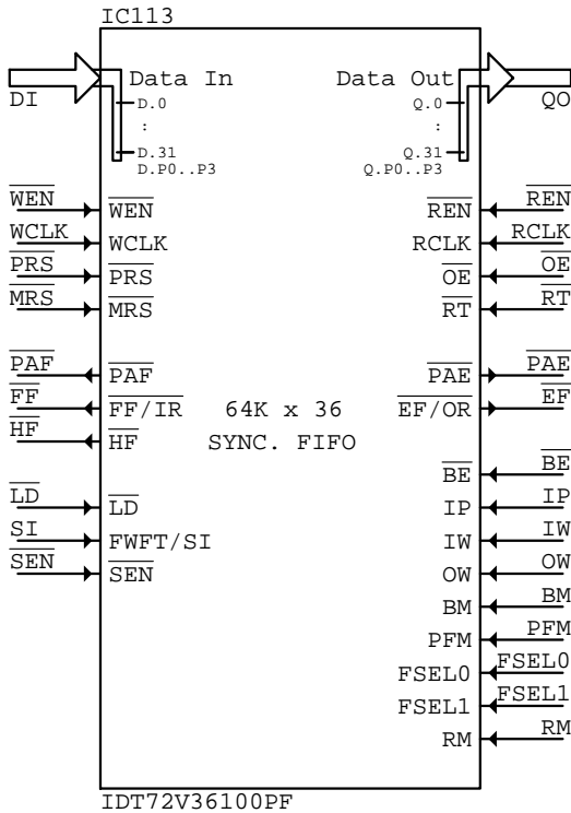
IDT72V36100PF_P IC???
