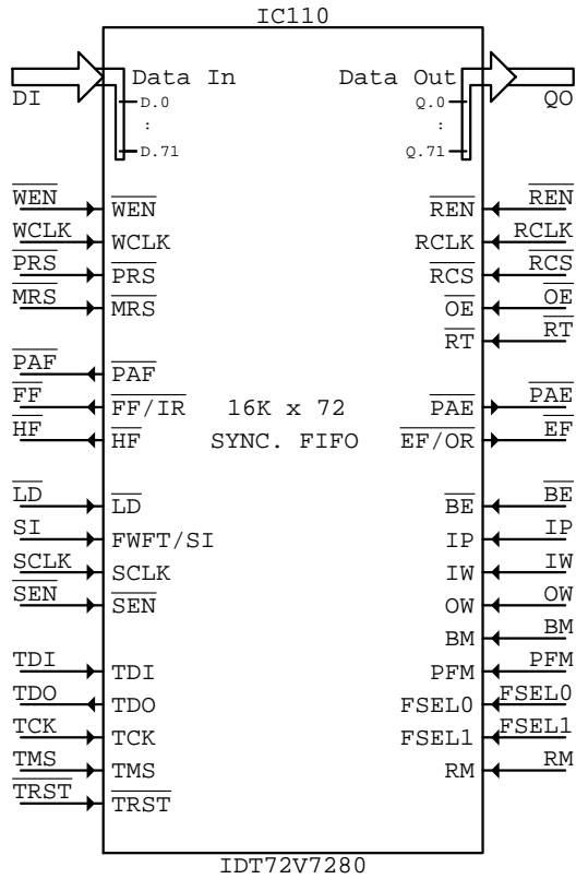
IDT72V7280
