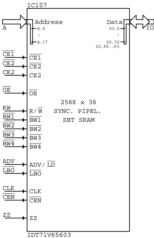
IDT71V65603 IC???
