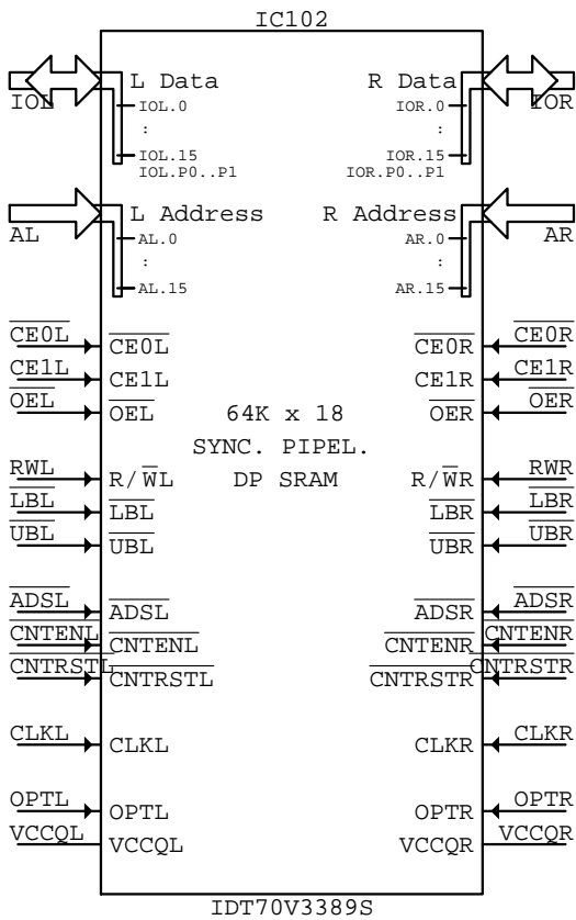
IDT70V3389 IC???
