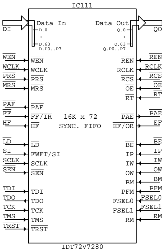
IDT72V7280
