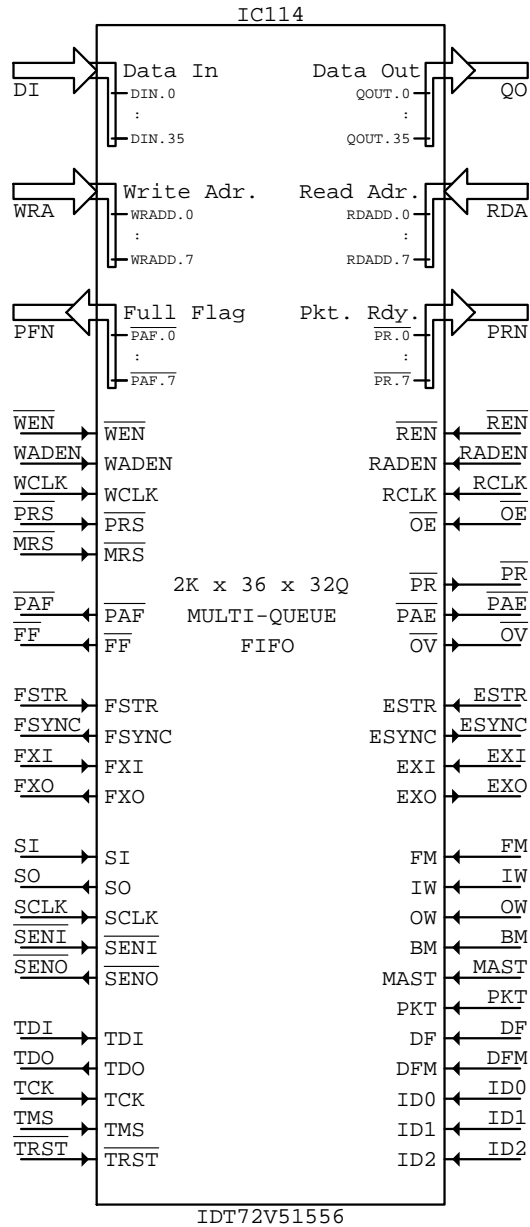
IDT72V51556 IC???
