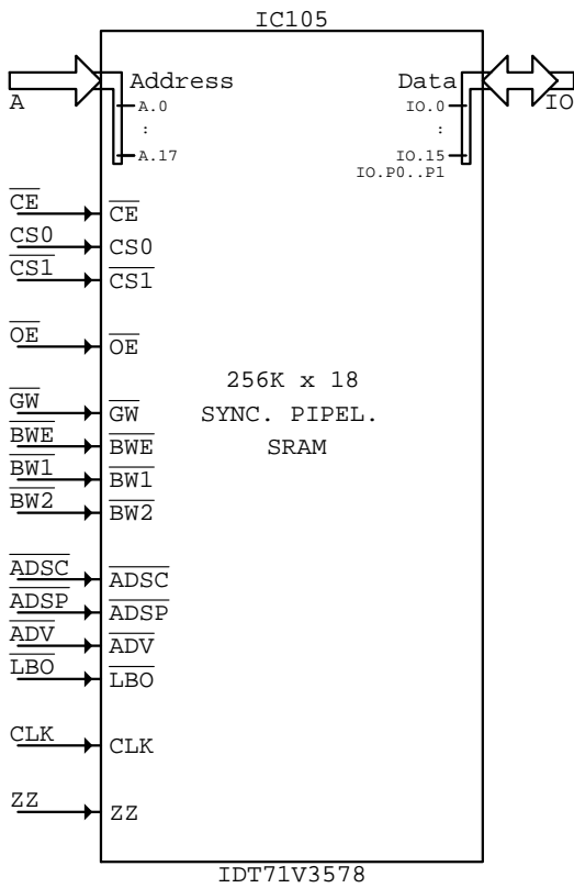
IDT71V3578 IC???
