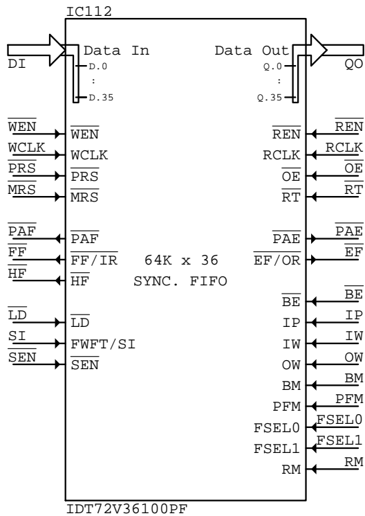
IDT72V36100PF
