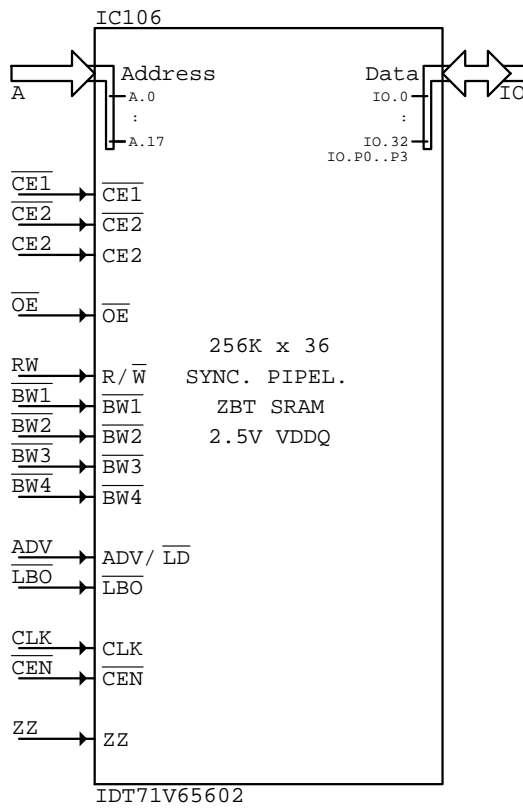
IDT71V65602 IC???
