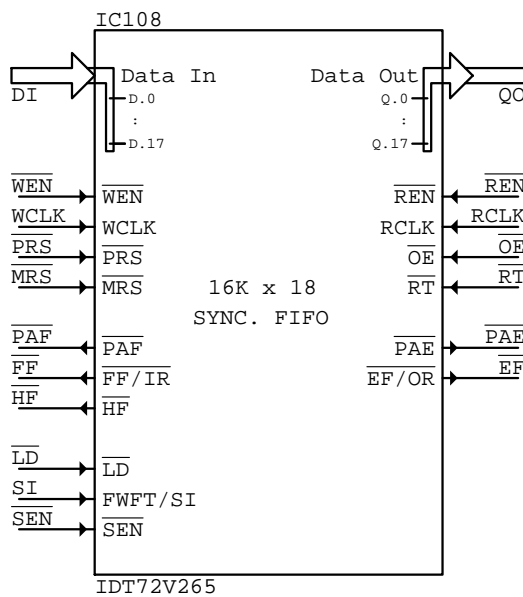
IDT72V265 IC???
