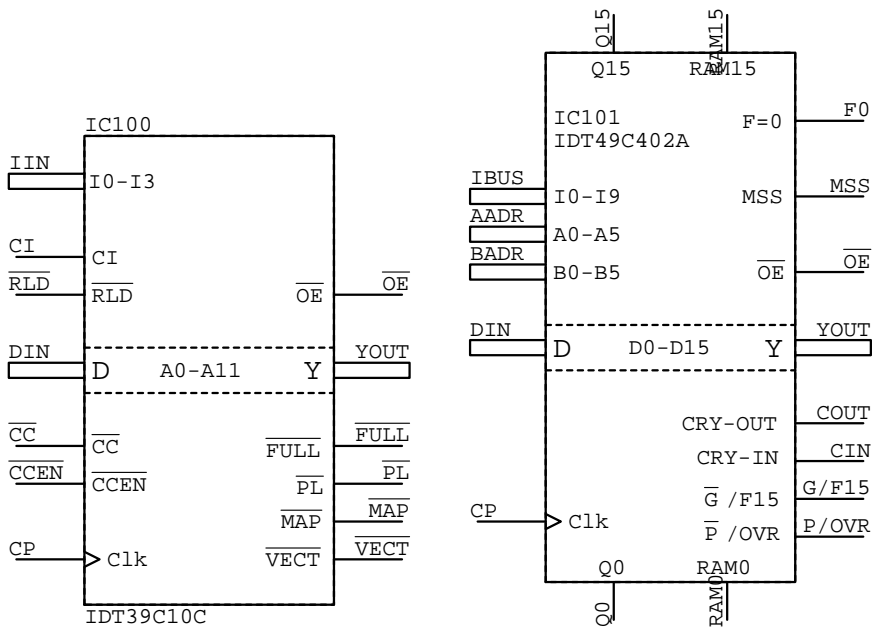
IDT39C10C IC???
