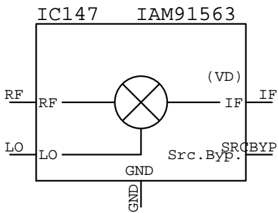
IAM91563 IC???
