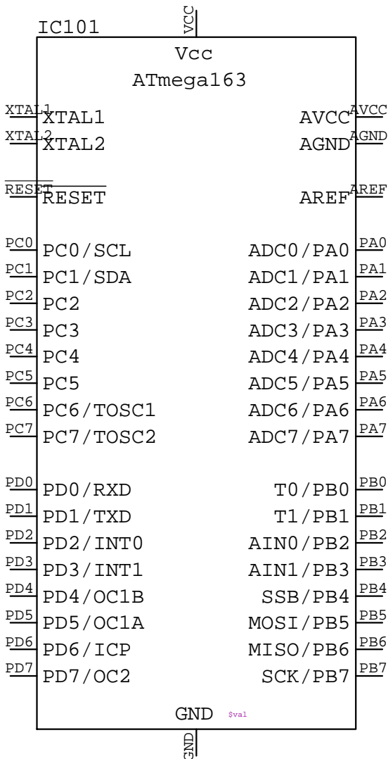
ATMEGA163 IC???
