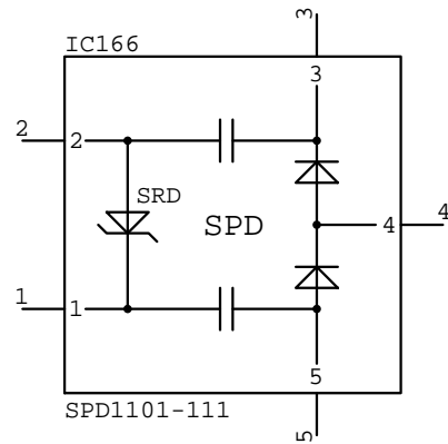
SPD1101 IC???
