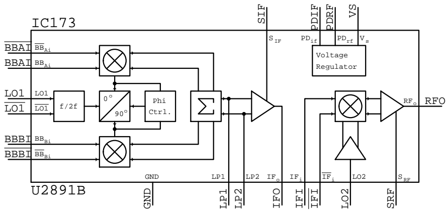
U2891B IC???
