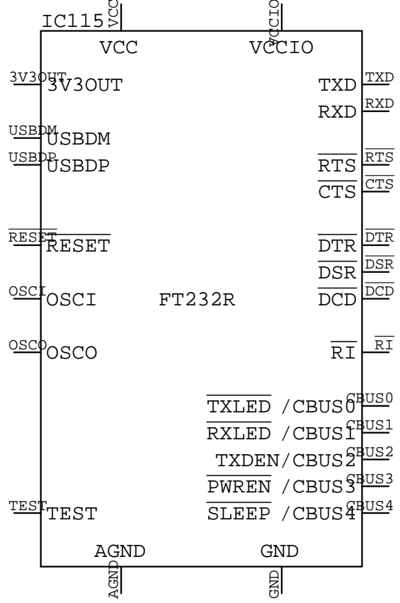
FT232RL IC???
