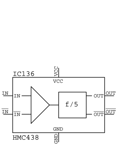
HMC438 IC???
