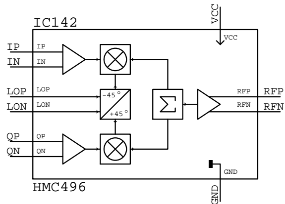
HMC496 IC???
