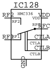
HMC336 IC???
