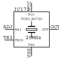
TCXO_N2720 IC???
