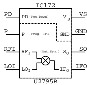
U2795B IC???
