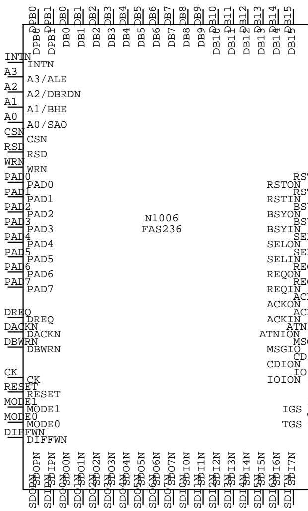
FAS236 N????
