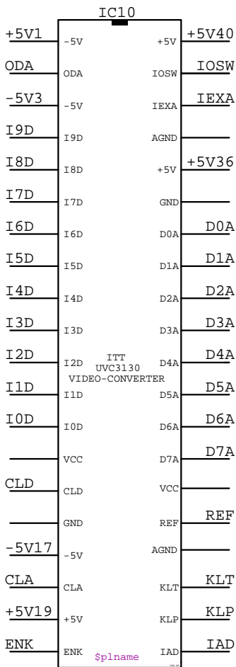
UVC3130 IC???
