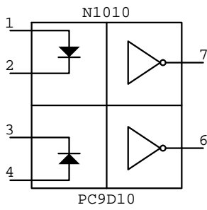
PC9D10 N????
