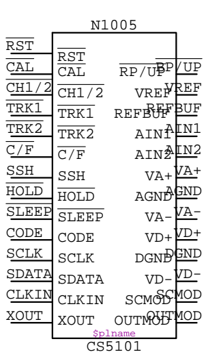
CS5101 N????
