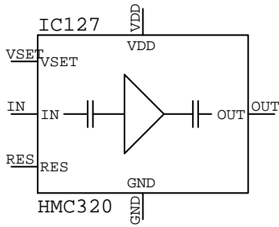
HMC320 IC???
