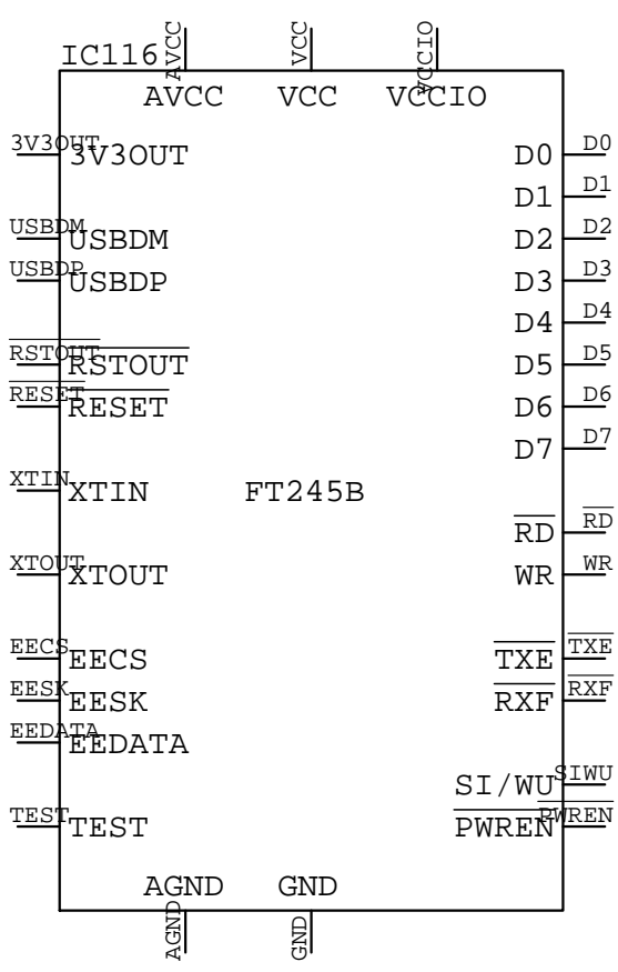
FT245B IC???
