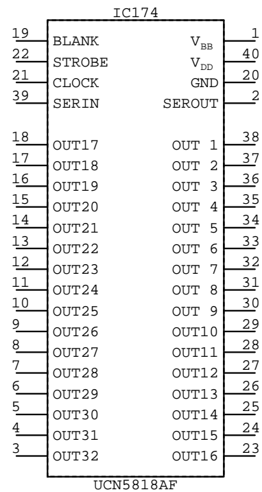
UCN5818AF IC???
