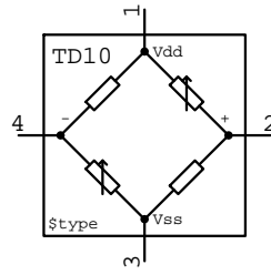
PRESSTRD TD??
