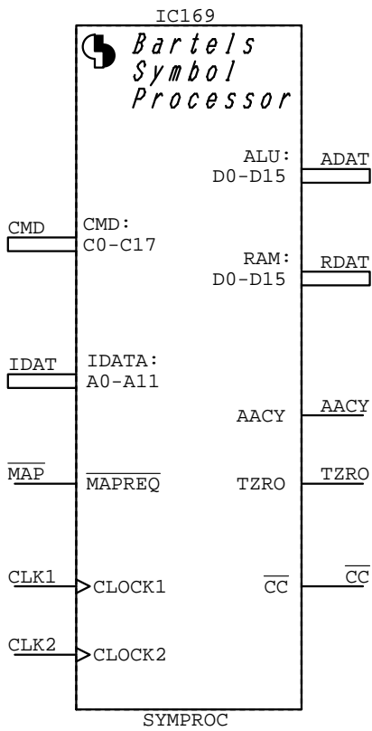
SYMPROC IC???
