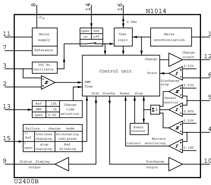
U2400B N????
