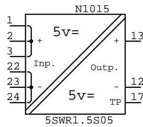
WDCDC_5SWR15S05 N????
