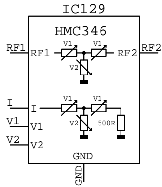
HMC346 IC???
