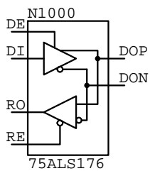
75ALS176 N????
