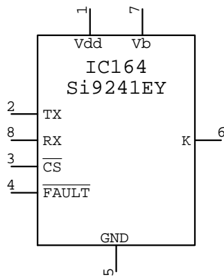
SI9241EY IC???
