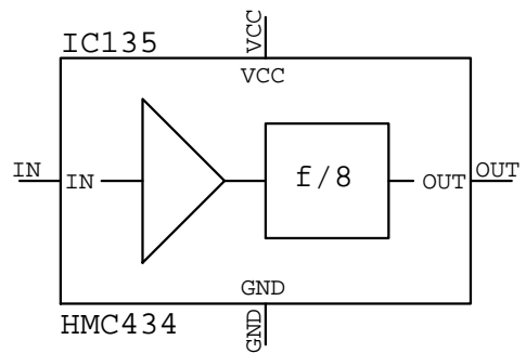
HMC434 IC???
