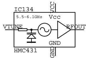
HMC431 IC???
