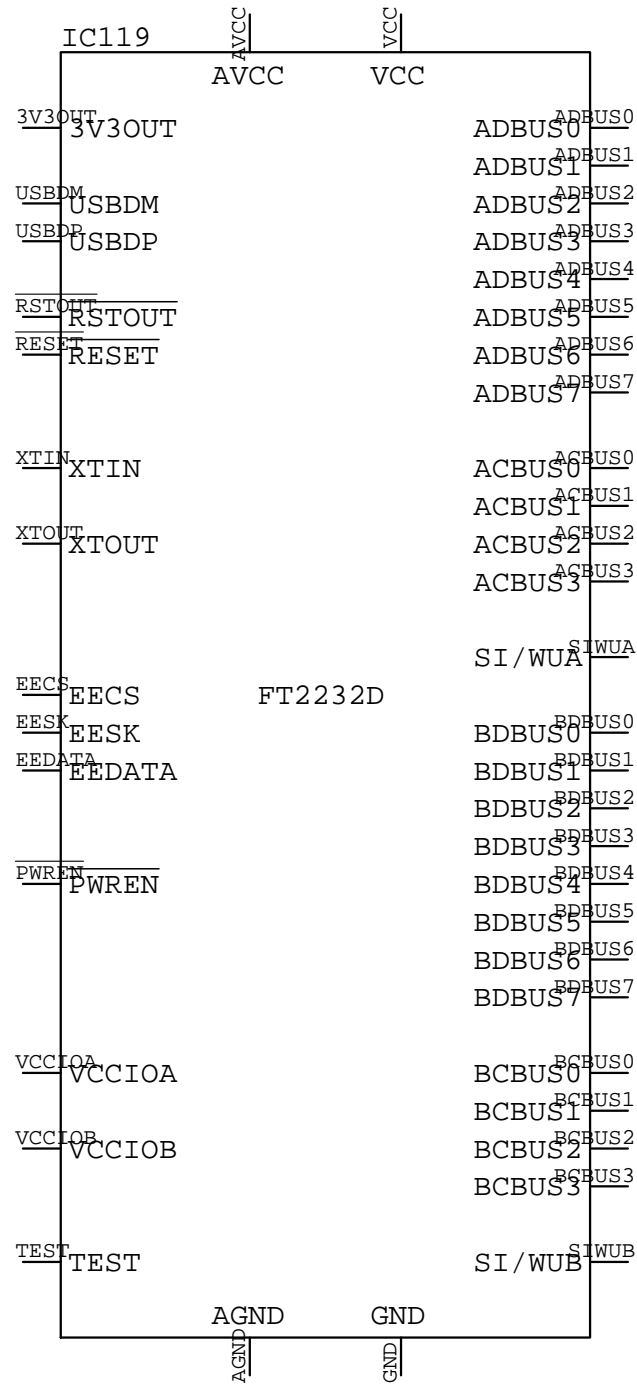
FT2232D IC???
