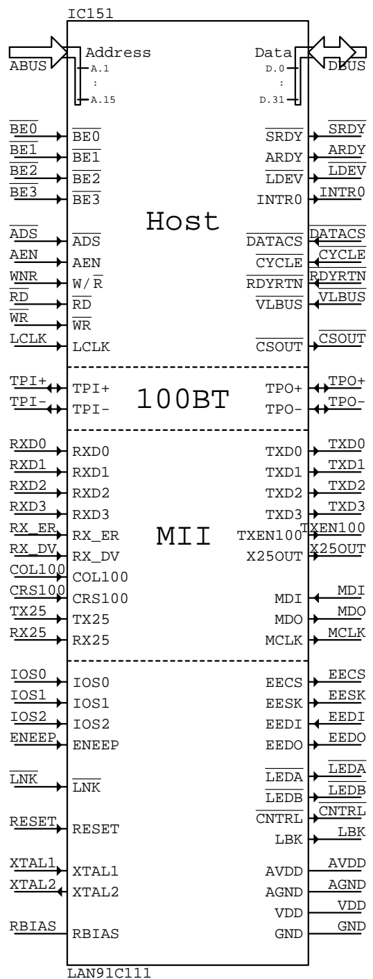
LAN91C111 IC???
