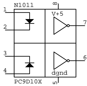
PC9D10X N????
