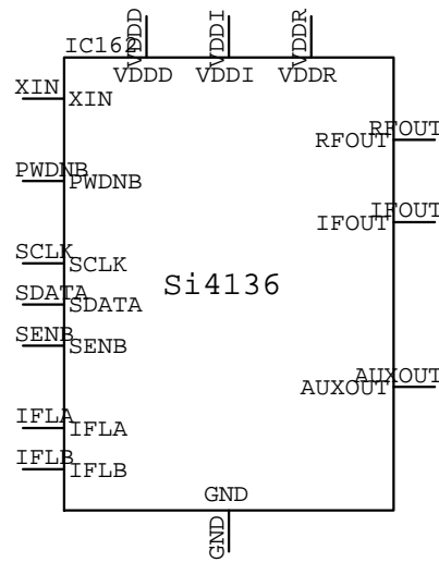
SI4136_BM IC???
