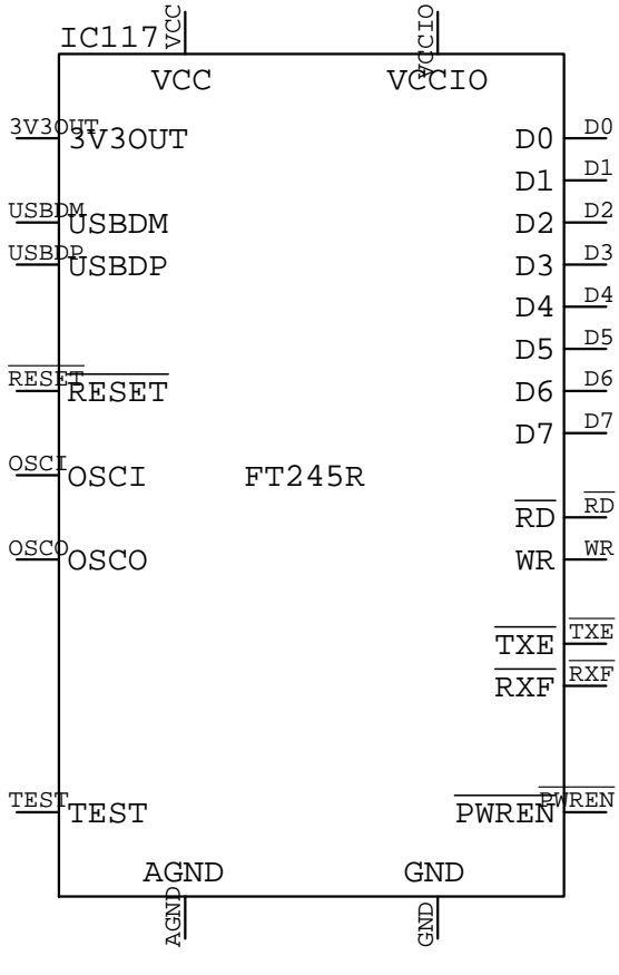
FT245RL IC???
