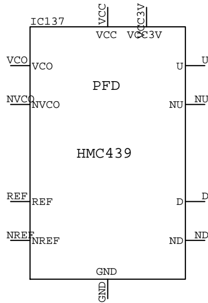
HMC439 IC???
