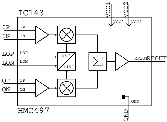
HMC497 IC???
