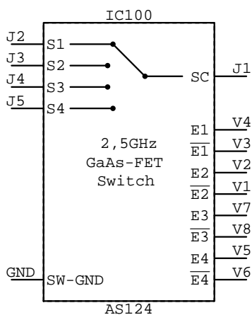
AS124 IC???
