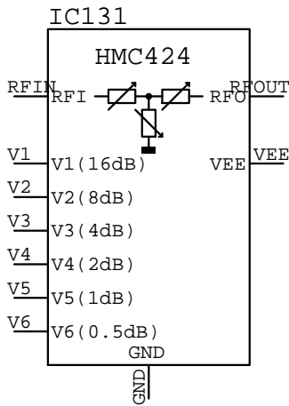
HMC424 IC???
