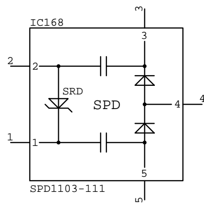
SPD1103 IC???
