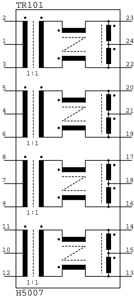
PULSE_H5007 TR???
