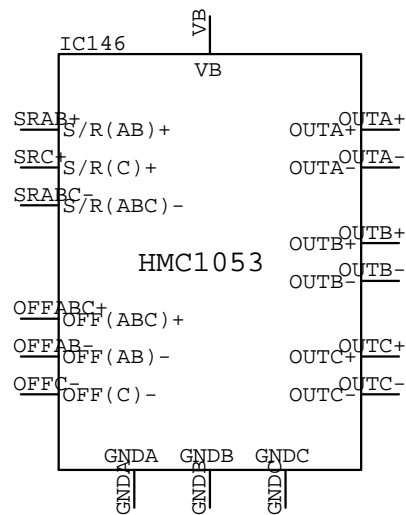
HMC1053 IC???
