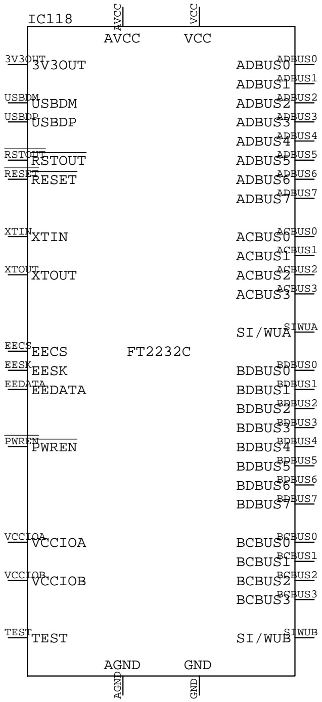
FT2232C IC???
