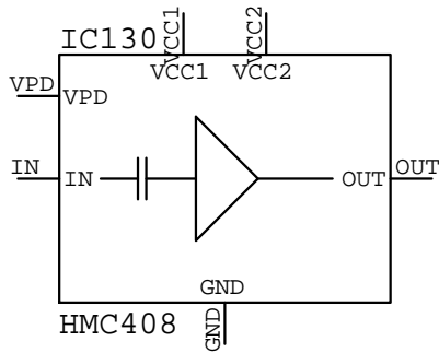
HMC408 IC???
