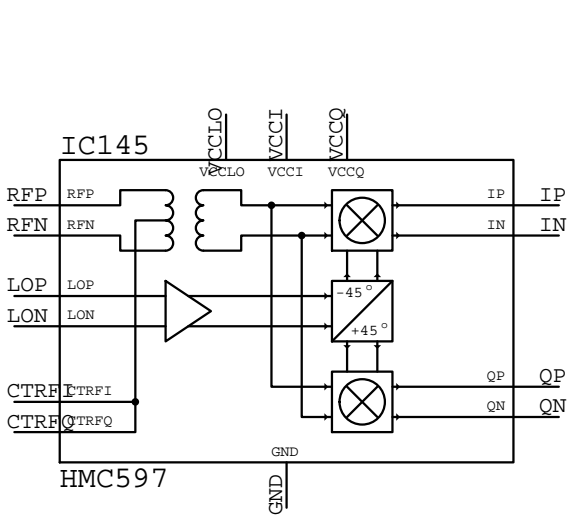
HMC597 IC???
