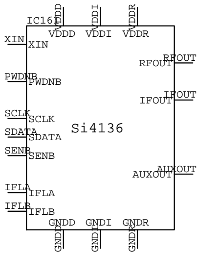
SI4136 IC???
